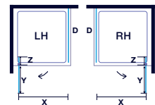
Pivot Door with Side Panel
