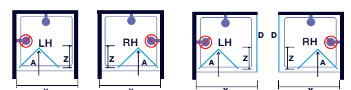
Bifold Door in Recess
